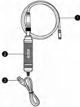
Figure 18-1 MaxiVideo Camera
