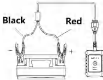
Figure 6-2 Connecting to a Battery
