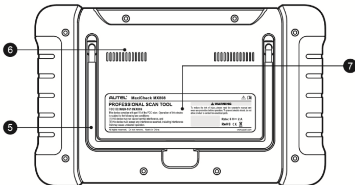
Figure 2-2 MaxiCheck MX808 Display Tablet Back View
